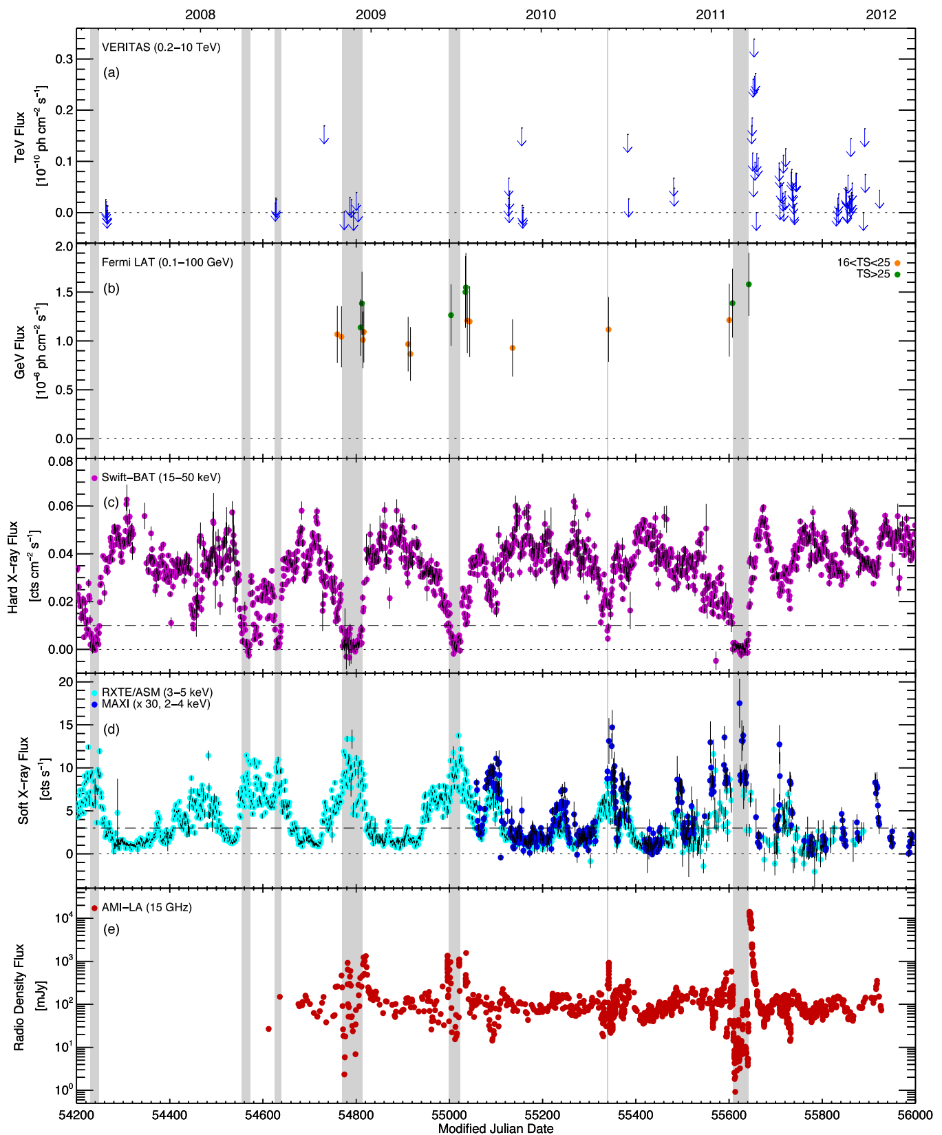
Figure 4. Multi-wavelength light curves of Cygnus X-3. Panels (a) TeV gamma ray. The VERITAS 99% C.L. integral ( E > 263 GeV) flux upper limits are shown for individual nights. (b) GeV gamma ray. The data points are color-coded by the detection significance: moderate significance ( 16 < TS < 25 ) in orange, and high significance ( TS > 25 ) in green. (c) Hard X-ray. (d) Soft X-ray. The ASM 3–5 keV measurements are shown in cyan and the MAXI 2–4 keV measurements in blue. Note that the MAXI flux values have been multiplied by 30 for clarity. (e) Radio. The AMI-LA 15 GHz measurements are shown. The shaded areas indicate the quenched state. The dot-dashed line in (c) and (d) shows roughly the threshold for transition into or out of the quenched state.
