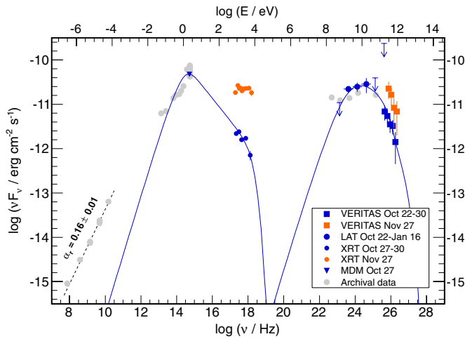
Figure 6. Spectral energy distribution of VER J0521+211 during the VERITAS detection. Optical, X-ray, GeV, and TeV data are shown for the low emission state (blue markers) and for the X-ray and TeV flare on 2009 November 27 (orange markers). Archival data points are shown in gray: radio (Cohen et al. 2007; Gregory et al. 1996; White & Becker 1992; Jackson et al. 2007; Condon et al. 1998), infrared (Wright et al. 2010; Cutri et al. 2003), optical (Monet et al. 2003; Drake et al. 2009), and gamma rays (Nolan et al. 2012). Archival radio data at 15 GHz is from the OVRO program ( http://www.astro.caltech.edu/ovroblazars ) and was obtained following Richards et al. (2011). Optical and infrared data are corrected for Galactic extinction using Schlafly & Finkbeiner (2011). A dashed black line shows the fit of the radio data to a power law with F_\nu \propto \nu^{-\alpha} . The solid blue curve represents a one-zone SSC emission model with parameters adjusted to describe the low-state data, assuming z = 0.1 . Radio data points are not reproduced by the model, as they are expected to sample outer regions of the blazar jet, where the emission becomes optically thin to radio waves.
