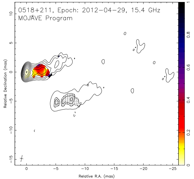
Figure 7. 15 GHz MOJAVE VLBA composite image of RGB J0521.8+2112 on 2012 April 29. The top left image shows contours of total intensity, with fractional linear polarization overlaid in color scale. The bottom right image shows contours of linear polarization, plus a single outermost contour of total intensity. Electric polarization vector directions are plotted as equal-length ticks. The contour levels for total intensity are 0.5 mJy beam -1 in steps of 2, while those for polarized intensity are for 0.7 mJy beam -1 in steps of 2. The restoring beam is indicated in the bottom left corner, and has Gaussian FWHM dimensions 1.15 by 0.57 mas, with major axis at -11.4^\circ from north.
