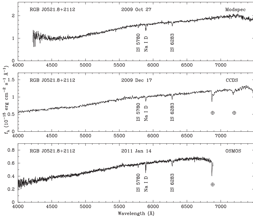
Figure 5. Optical spectra of RGB J0521.8+2112 obtained on the 2.4 m Hiltner telescope of the MDM Observatory. The Modspec spectrum was obtained with an exposure of 2 \times 600 s and a resolution of 4 Å. The exposures for the CCDS and OSMOS spectra were 3 \times 1800 s with resolution of 8 Å and 3 Å, respectively. Galactic interstellar absorption lines are labeled with their wavelength, including the Na I D doublet and diffuse interstellar bands at 5780 Å and 6283 Å. These are relatively prominent because of the low Galactic latitude of -8.7 and the corresponding visual extinction A_V = 1.9 (Schlafly & Finkbeiner 2011) to the source. Telluric absorption by \text{O}_2 and \text{H}_2\text{O} are indicated in the CCDS and OSMOS spectra; in the case of Modspec they were corrected using the spectrum of a featureless B star.
