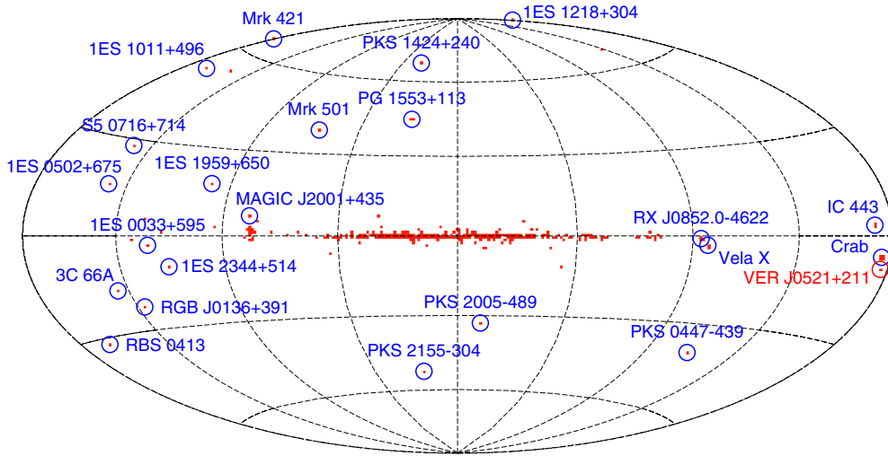
Figure 1. Map, in Galactic coordinates, showing the arrival directions of all diffuse-class photon events 41 with zenith angle < 105^\circ recorded by Fermi -LAT between 2008 August 4 and 2009 August 25 with reconstructed energies greater than 30 GeV. The events are binned in 1^\circ bins, and bins containing at least five events are shaded red. Known TeV sources coincident with shaded bins are indicated in regions where source confusion or diffuse background is not an issue.
