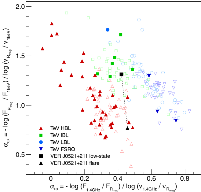
Figure 8. Spectral slopes of the synchrotron component for gamma-ray blazars. The effective spectral indices \alpha_{ro} and \alpha_{ox} are defined in the usual way between 1.4 GHz, 6590 Å, and 1 keV. SED classifications for the 47 known TeV blazars (filled markers) are taken from TeVCat (Wakely & Horan 2008). Multiband fluxes are obtained from Massaro et al. (2009) with the exceptions of RX J0648.7+1516, HESS J1943+213, and MAGIC J2001+435 (Condon et al. 1998; Monet et al. 2003; Voges et al. 1999; Bassani et al. 2009). Empty markers show GeV-detected blazars from Nolan et al. (2012) present in Massaro et al. (2009). VER J0521+211 is pictured in a “low-state” (2009 October 22–30) showing a spectral shape characteristic of IBLs, and in “flare” (2009 November 27), when it shows HBL-like properties.
