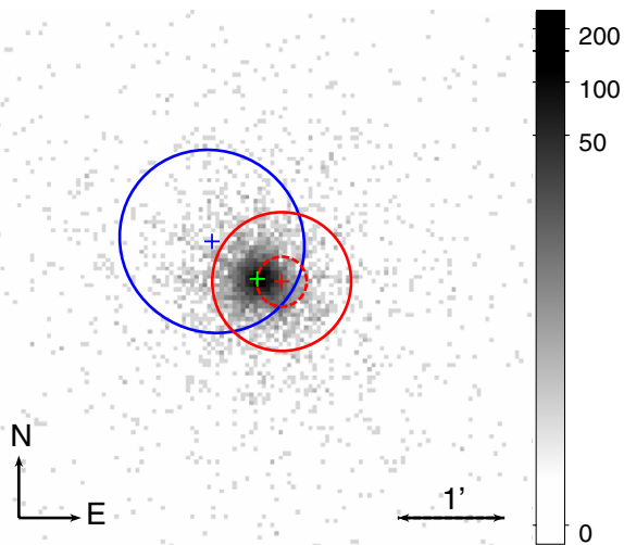
Figure 4. Swift /XRT cumulative counts map in the 0.3–10 keV band, zoomed-in at the location of VER J0521+211. The field is 5' \times 5' , with gray code indicating counts on a logarithmic scale. The green cross indicates the best-fit centroid to the Swift /XRT data. The red cross shows the position of VER J0521+211 with red dashed circle indicating the VERITAS 68% statistical location error and red-solid line showing statistical and systematic error. The blue ellipse displays 68% error contour of 2FGL J0521.7+2113 as measured by Fermi -LAT (Nolan et al. 2012).
