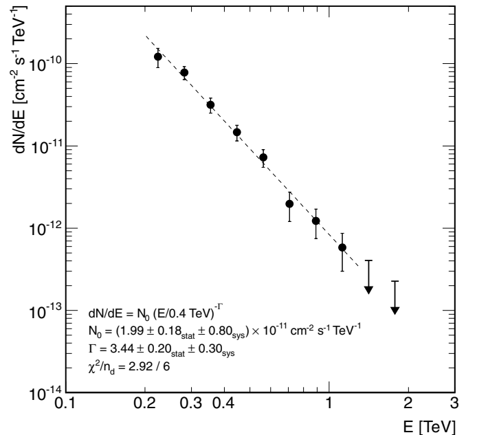
Figure 2. Time-averaged differential photon spectrum of VER J0521+211, obtained during VERITAS observations between MJD 55126 (2009 October 22) and MJD 55212 (2010 January 16). Upper limits at 95% confidence level are shown for the two highest energy points, where the significance is < 2\sigma .
