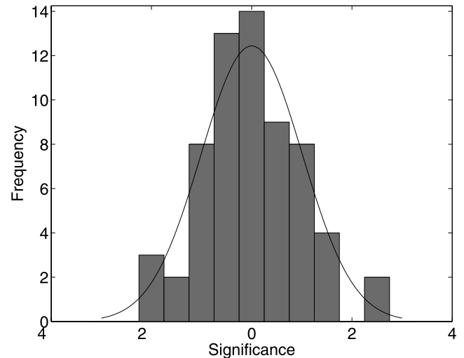
FIG. 2.—Significance of the deficit or excess in the detected count rate from each of the 29 BL Lac objects for each season during which they were observed. This distribution has a mean of 0.005 and standard deviation of 0.976. The black curve shows the expected shape if the significances were normally distributed. This curve fits the data at the 95% confidence level.
