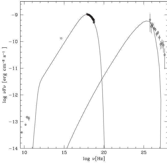
FIG. 11.—Spectral energy distribution of Mrk 421. It was derived from the high-flux data group (see text). The solid line shows the best fit to the data with a one-zone SSC model (see text): \delta = 14 , B = 0.26 G, R = 0.7 \times 10^{16} cm, w_e = 0.086 ergs cm ^{-3} , p_1 = 2.05 , p_2 = 3.4 , \log(E_b) = 11.0 , \log(E_{\min}) = 6.5 , and \log(E_{\max}) = 11.6 . All energies ( E 's) are in units of eV. Note large deviations at both very low and high frequencies.
