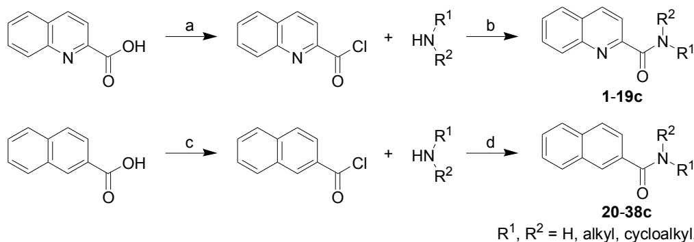
Scheme 1. Synthesis of quinoline-2-carboxanilides 1–19c and naphthalene-2-carboxamides 20–38c .
