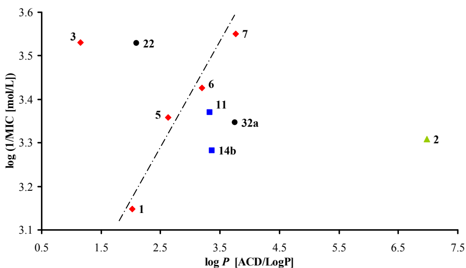
Figure 4. Dependence of in vitro average antimycobacterial activity against Mycobacterium sp. ( \log 1/\text{MIC} [mol/L]) on lipophilicity expressed as \log P of the studied quinaldinamides. (red rhomb = branched alkyl quinaldinamides, green triangle = unbranched long-chain alkyl quinaldinamide, blue square = aromatic quinaldinamides, black point = naphthamides).
