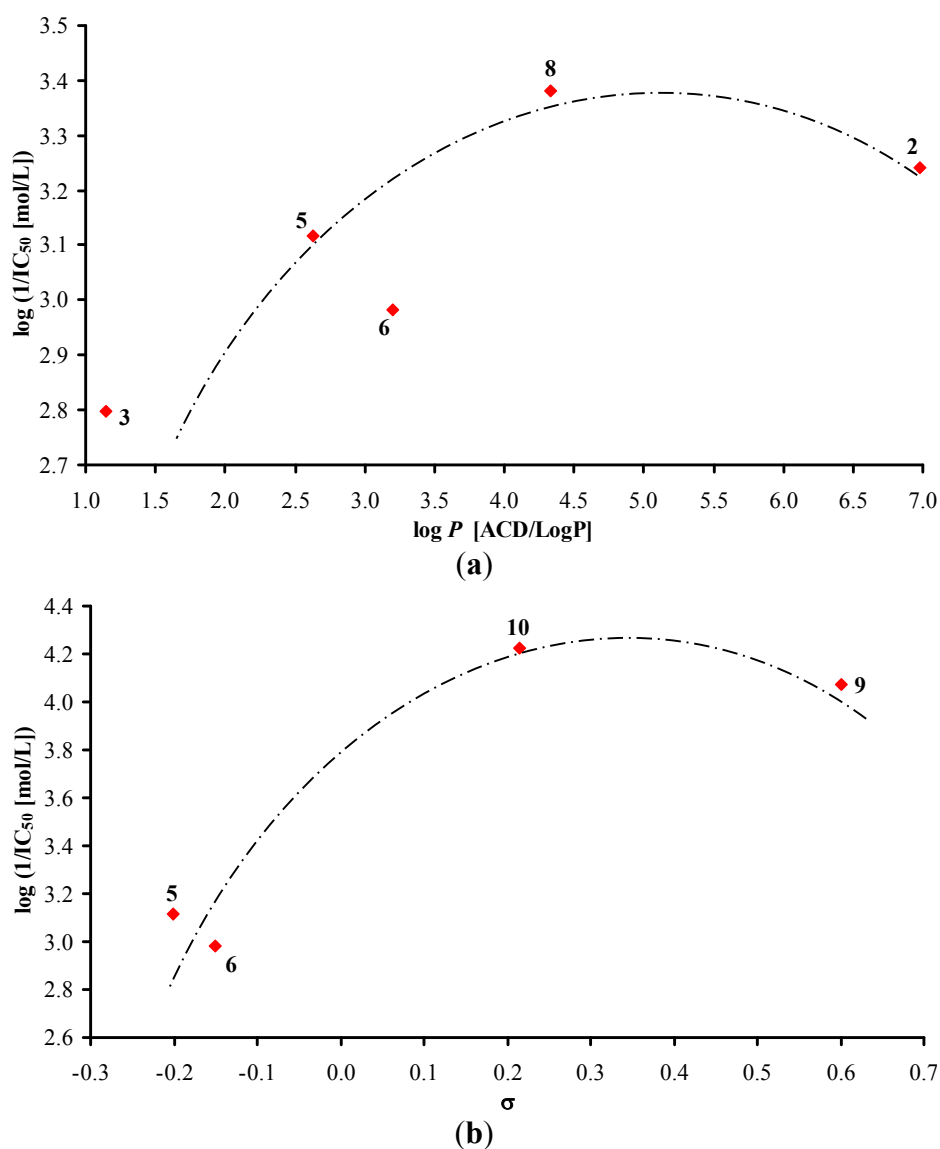
Figure 1. Relationships between PET inhibition \log(1/IC_{50}) [mol/L] in spinach chloroplasts and lipophilicity (a) or N -substituent electronic \sigma parameters (b) of studied compounds 1–10 .
