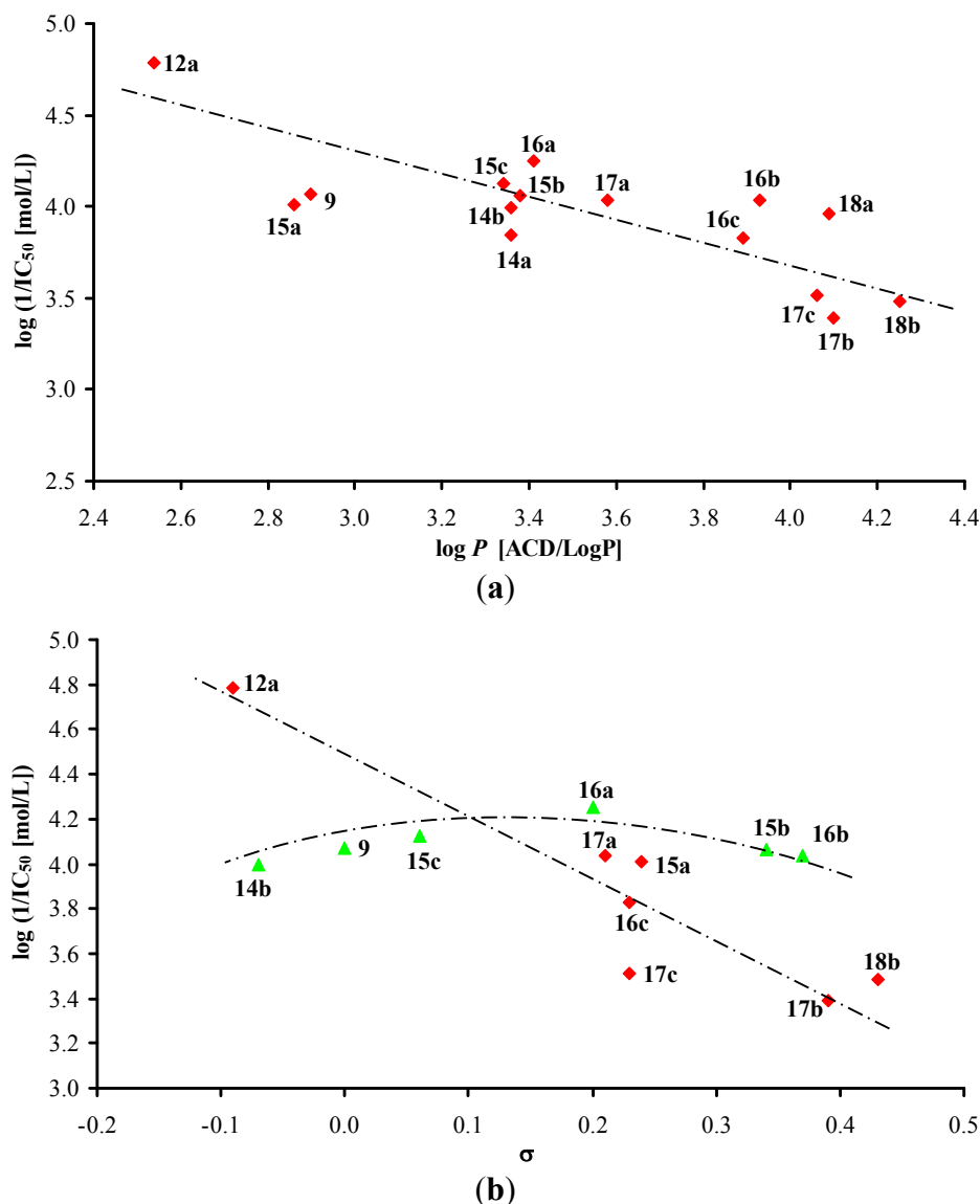
Figure 2. Relationships between PET inhibition \log(1/IC_{50}) [mol/L] in spinach chloroplasts and lipophilicity (a) or N -substituent electronic Hammett's \sigma parameters (b) of studied compounds 9 , 12a–19c .
