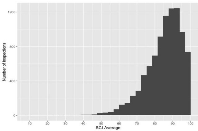
Figure 6: Graph showing distribution of BCI Average for the new inspections which use the BCI inspection process.
