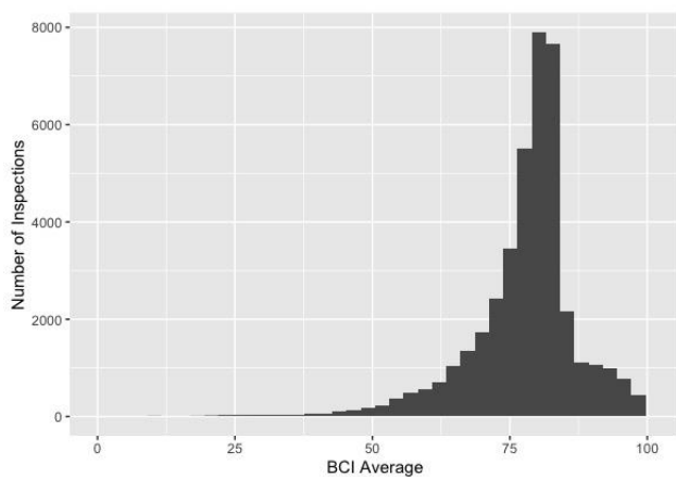
Figure 9: Graph showing distribution of BCI Average for all inspections.
