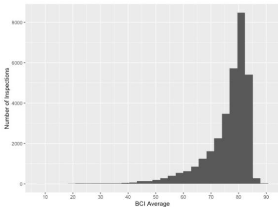
Figure 7: A graph showing the distribution of the BCI Average for the legacy inspections.
