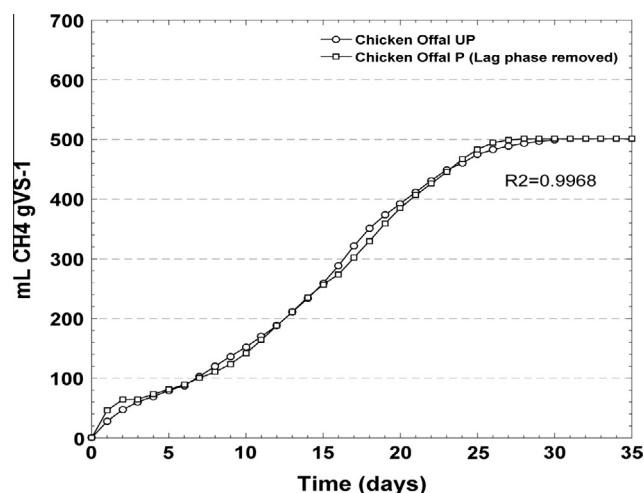
Fig. 5. Comparison of cumulative specific methane curves for UP chicken and P chicken after removal of 15 day lag phase observed between day 4 and 19.
